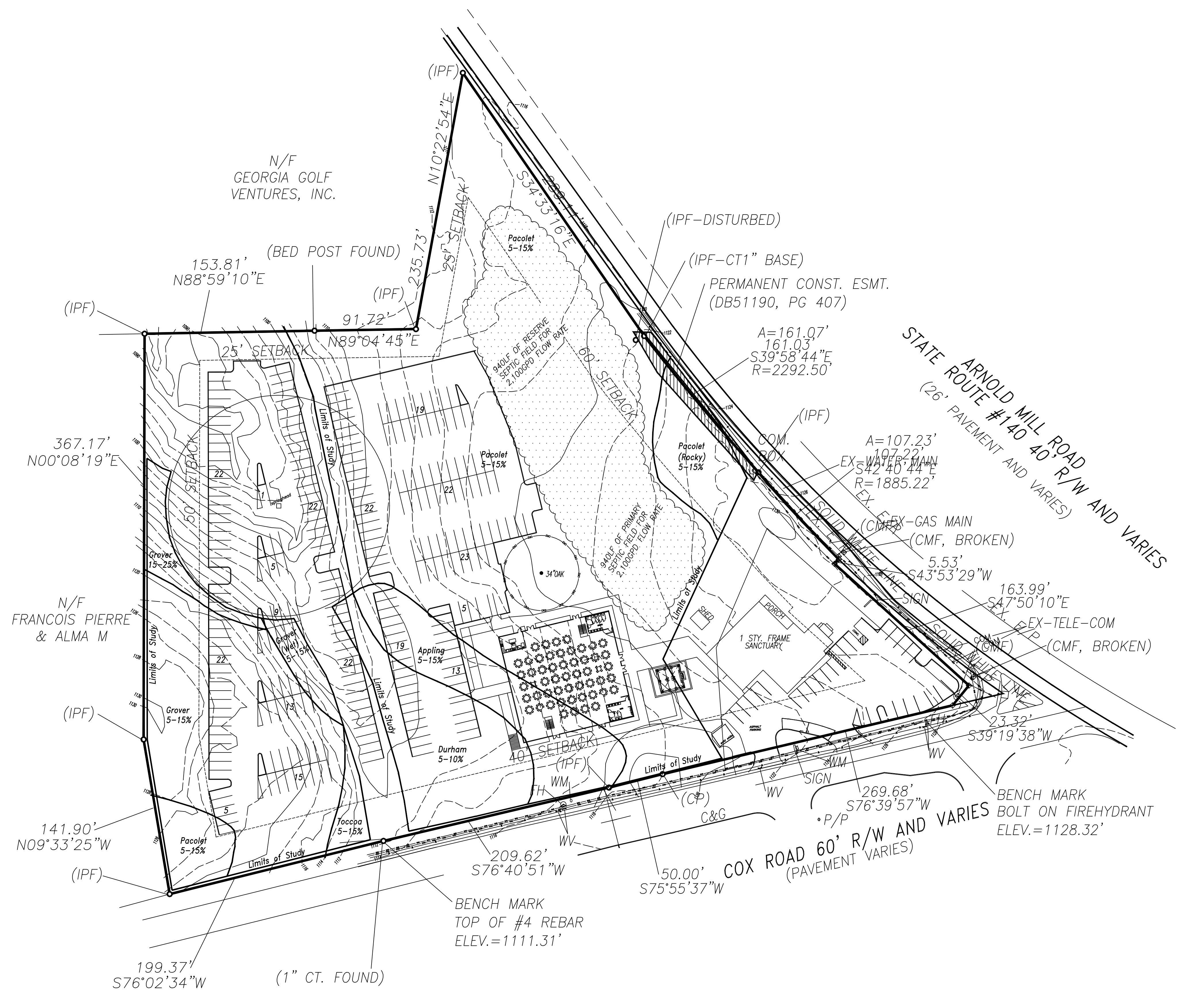
1 ARCHITECTURAL SITE PLAN 1" = 50'-0"
